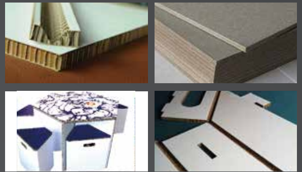
IECHO V-CUT The V-Cut tool is the perfect tool for pre-producing complex structural designs from foam core or sandwich board materials. The tool can be set for cutting 5 different angles for different cutting requests. The 5 different angles are 0°, 15°, 30°, 45° respectively.
